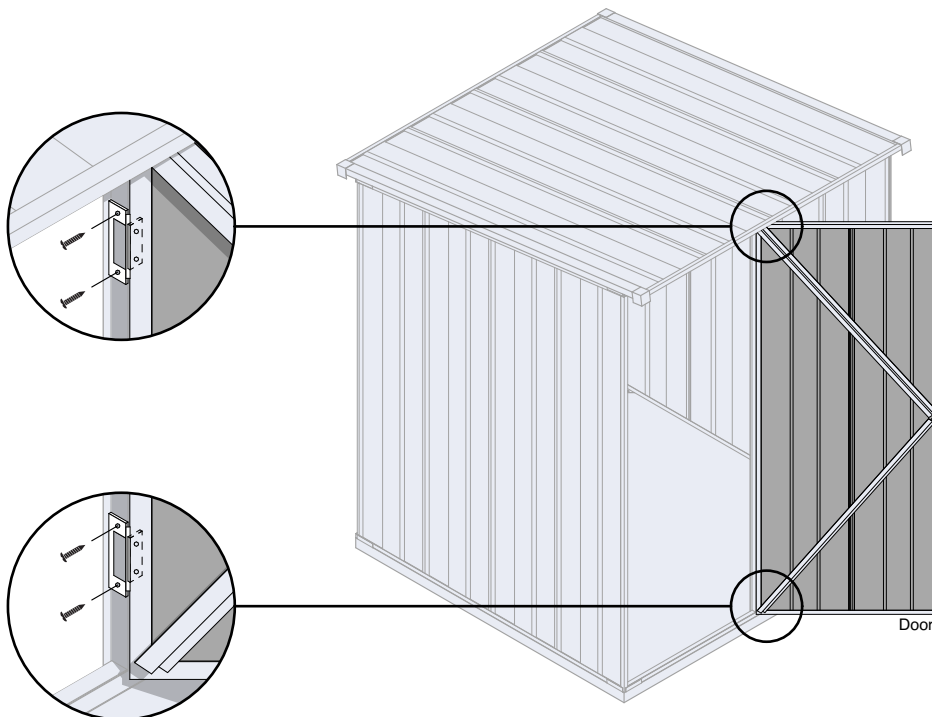
Bolt (Outside)
